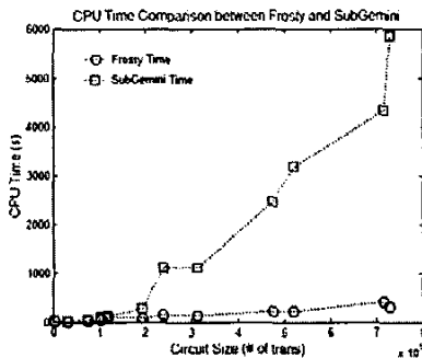
Figure 12. FROSTY and SubGemini CPU time comparison.
