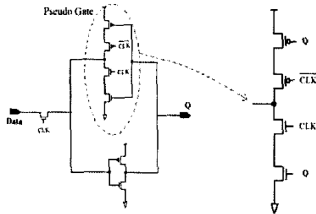
Figure 3. Pseudo CMOS Gate.
