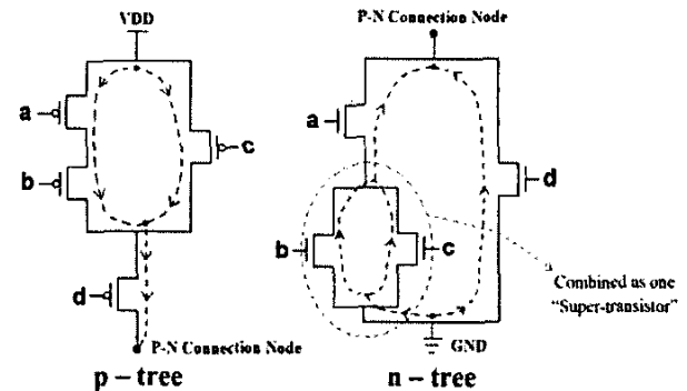
Figure 2. Group the channel-connected blocks.
