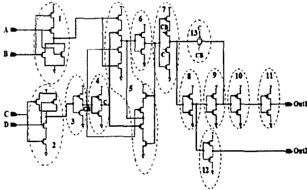
Figure 7. The object circuit after the gate recognition.
