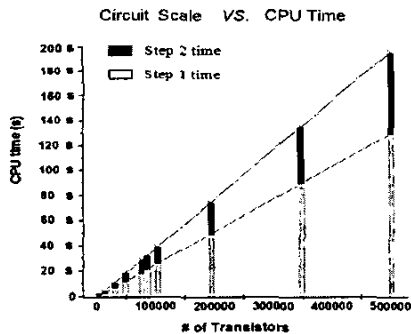
Figure 13. CPU time vs. circuit scale.
