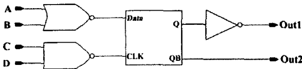
Figure 9. The extracted block-level structure.
