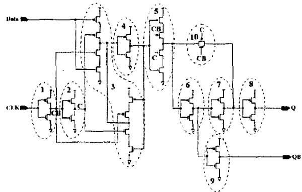
Figure 5. D flip-flop (DFF) circuit after gate recognition.
