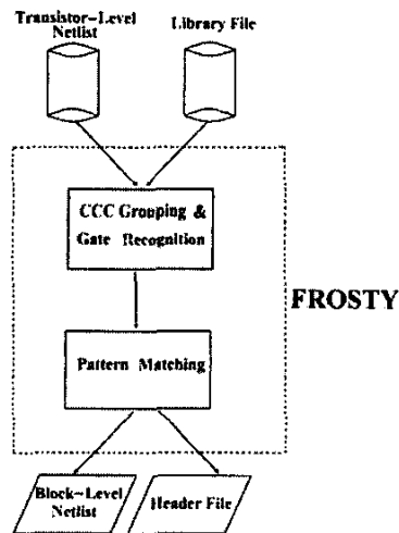
Figure 1. FROSTY flow and architecture.
