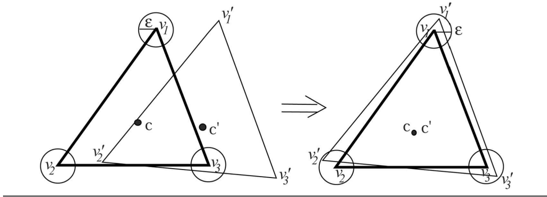
Figure 8 Parametric tolerance class \Delta(P, \epsilon) for feeding and procedure to check if a candidate part P is in the class
