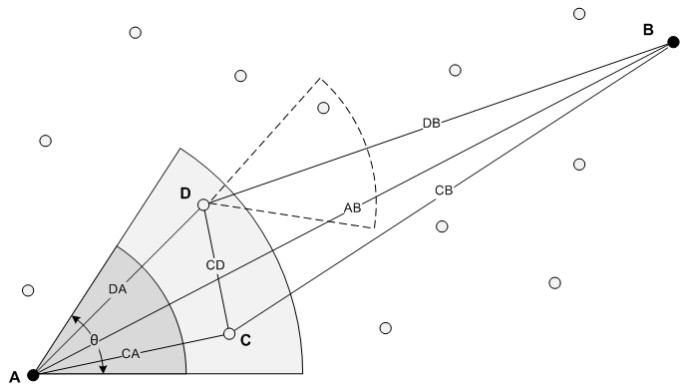
Figure 1: Illustration of the routing protocol: nodes within the transmitter's cone \theta are candidate relays.
