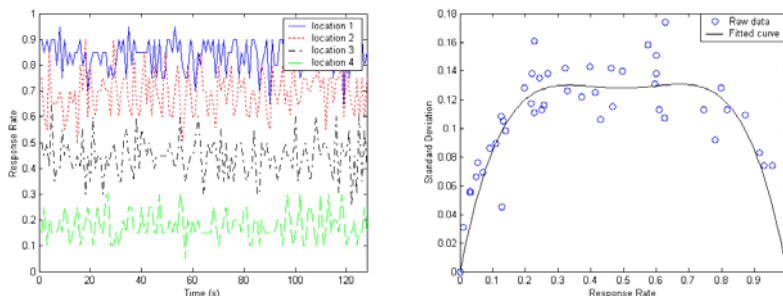
Fig. 1. Left: The response rate at 4 different distances, with N=20 . Right: The relationship between mean and standard deviation of response rate ( N=10 )
