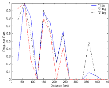
Fig. 3. Response rate as a function of distance from the reader, with a metal floor
