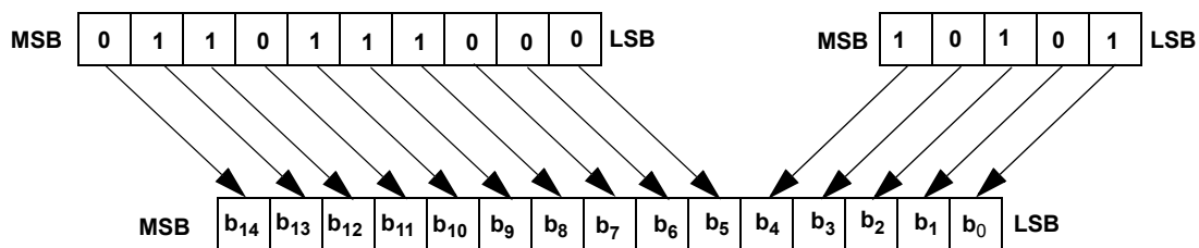
OFDMA randomizer initialization vector
