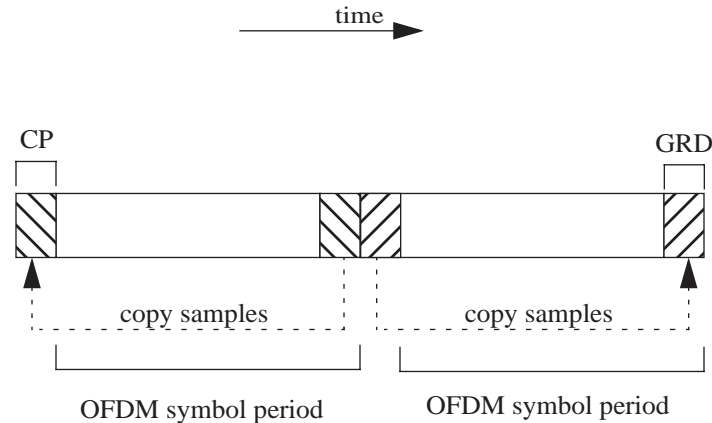
Figure 239—Initial-ranging/handover-ranging transmission for OFDMA
