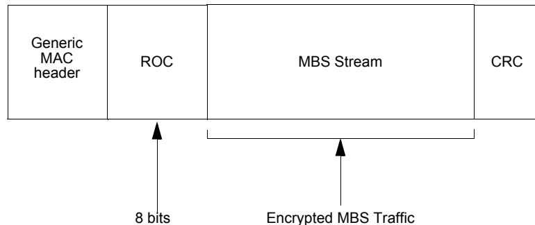
Figure 137a—MBS MAC PDU Ciphertext payload format
