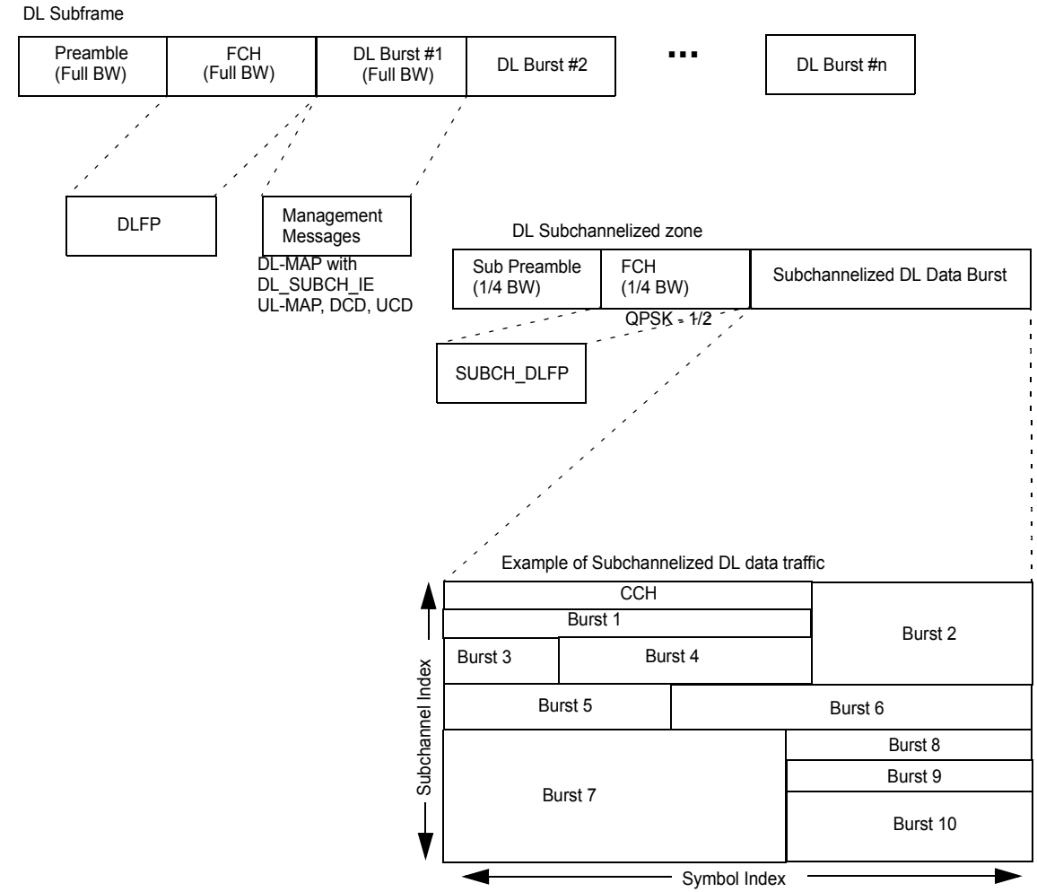
Figure 208a—Format of DL subchannelization zone
