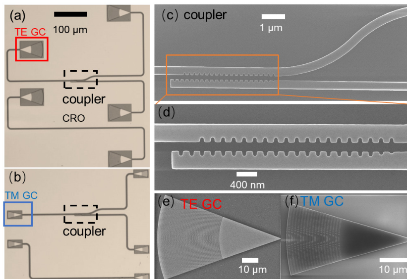
Ultra-compact subwavelength-grating-assisted polarization-independent directional coupler, as seen in “Ultra-Compact Subwavelength-Grating-Assisted Polarization-Independent Directional Coupler,” by H. Xie, et al. , p. 1538. (a), (b) Optical microscope images of two fabricated polarization-independent directional couplers. (c), (d) Scanning electron microscope images of the device and the zoom-in view of the coupling region. (e), (f) Scanning electron microscope images of the grating couplers.
